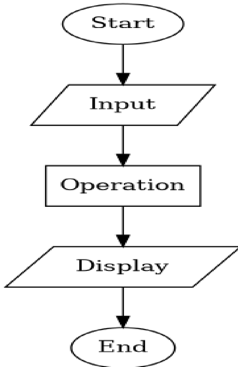
Figure 4.5 Trigonometry
